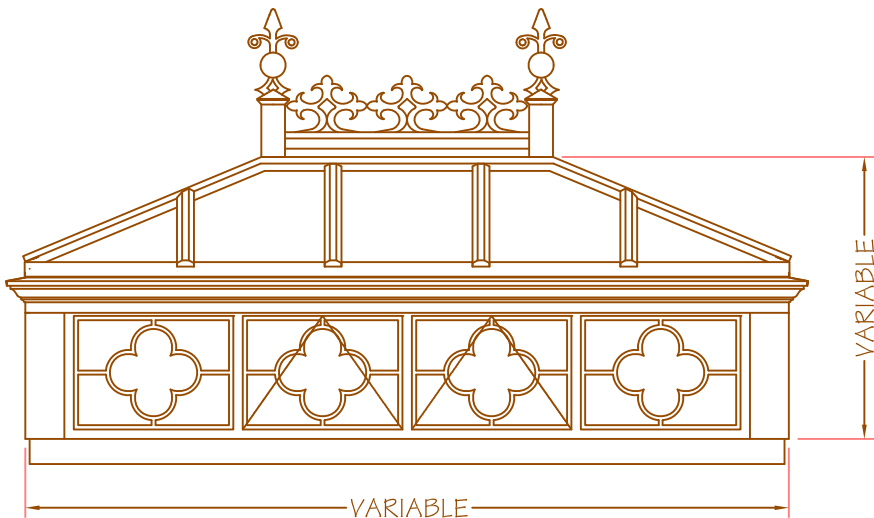
VARIABLE - LANTERN FRONT VIEW -
