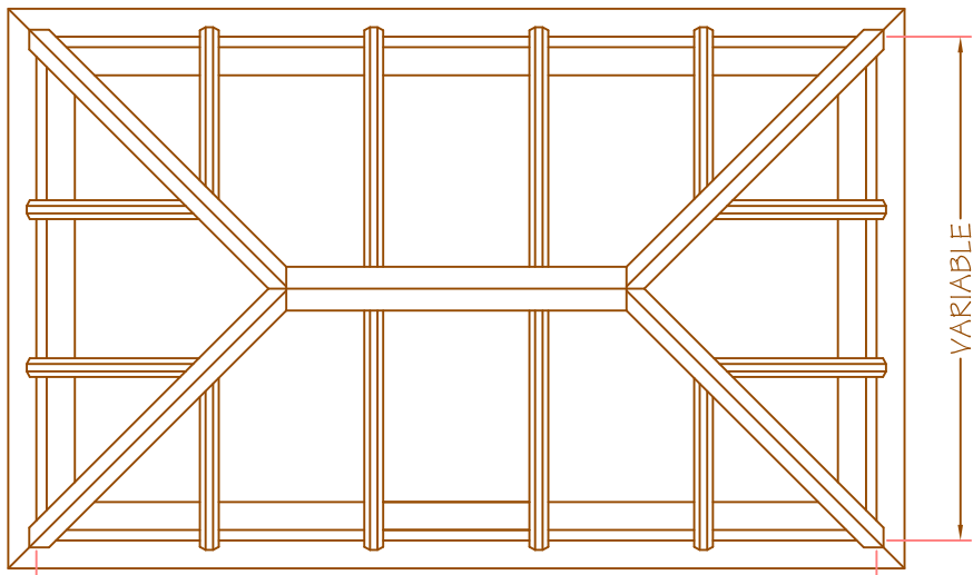
VARIABLE - ROOF PLAN -
