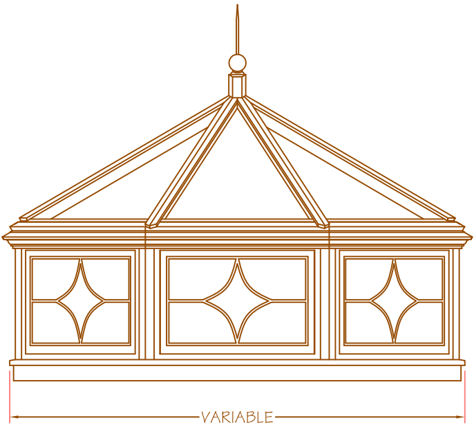
- LANTERN FRONT ELEVATION -
