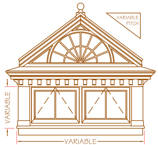
- VARIABLE - - LANTERN GABLE ELEVATION -
