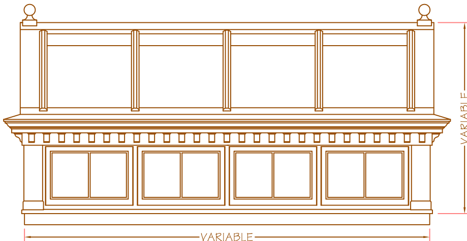
- VARIABLE - - LANTERN FRONT ELEVATION -
