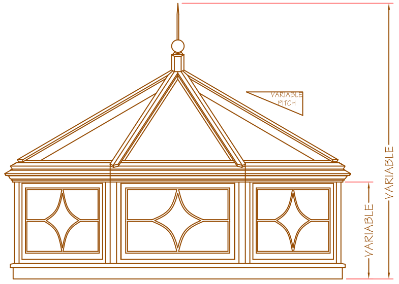
- LANTERN SIDE ELEVATION -
