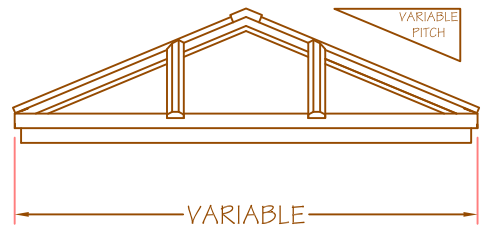
VARIABLE PITCH VARIABLE - SKYLIGHT ROOF VIEW -
