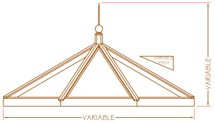
- SKYLITE ROOF ELEVATION -
